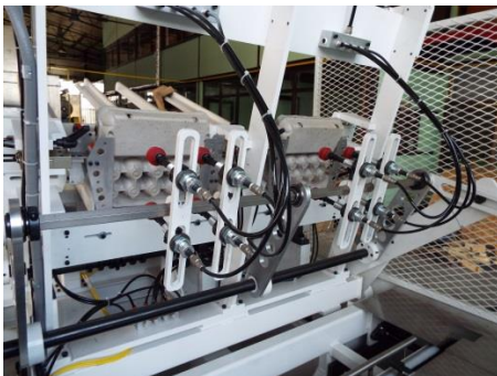
Automatic Stacker
